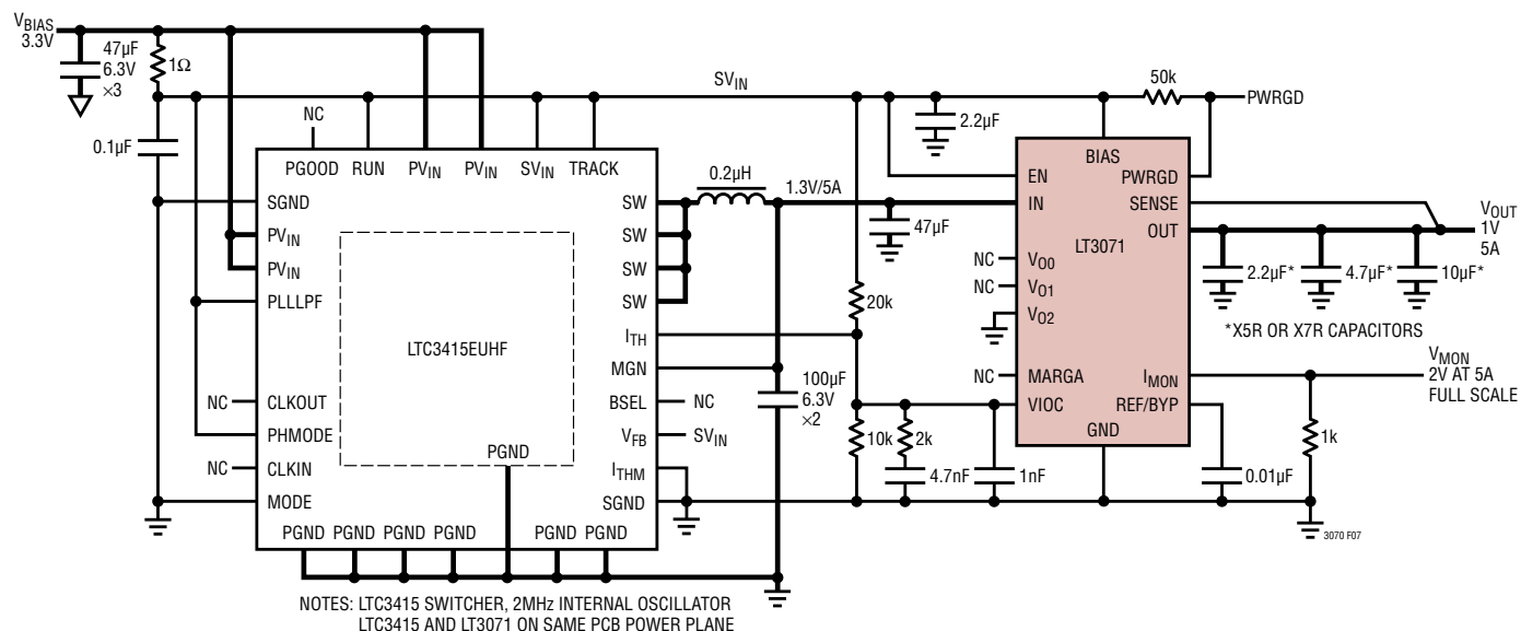
Figure 7. Regulator with VIOC Buck Control
